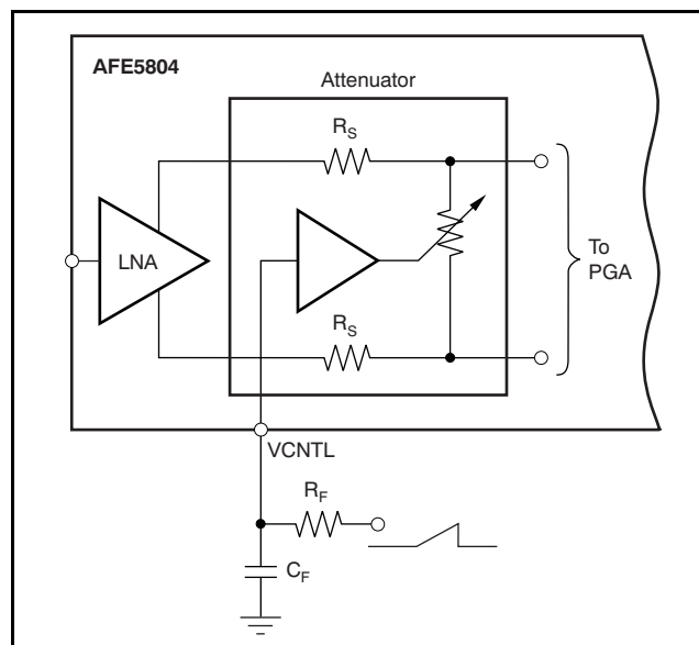
Figure 101. External Filtering of the V_{CNTL} Input
