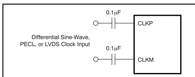
Figure 105. Differential Clock Driving Circuit ( \text{DIFF\_CLK} = 1 )
