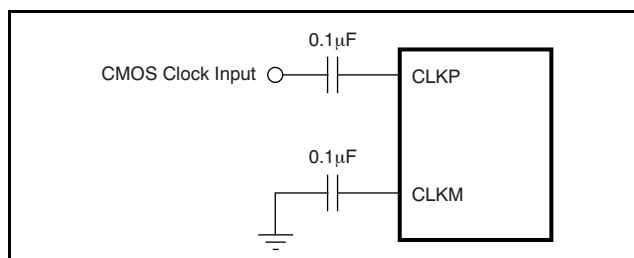
Figure 106. Single-Ended Clock Driving Circuit When \text{DIFF\_CLK} = 1
