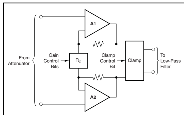
Figure 97. Post-Gain Amplifier (Simplified Schematic)
