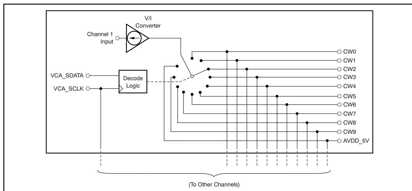
Figure 91. Basic CW Cross-Point Switch Matrix Configuration
