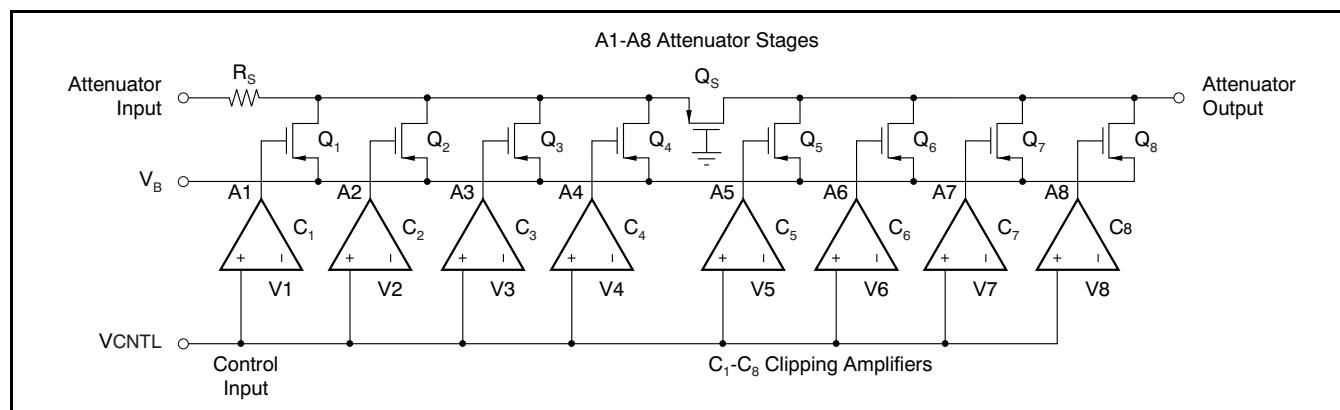
Figure 96. Voltage-Controlled Attenuator Simplified Schematic
