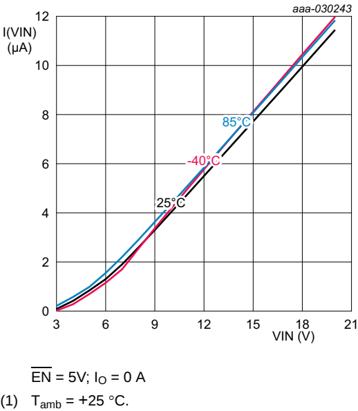
Fig 9. OFF-state quiescent current versus input voltage
