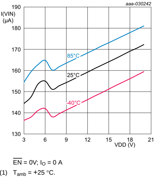
Fig 8. On-state quiescent current versus input voltage
