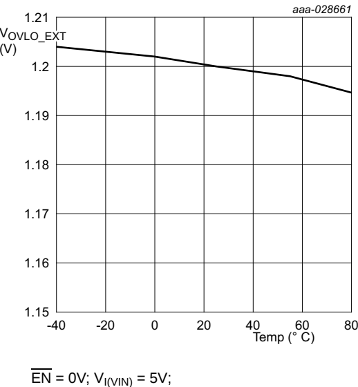
Fig 11. External OVLO set threshold versus temperature
