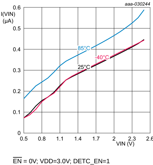
Fig 10. VIN pin leakage current in detection mode versus VIN voltage
