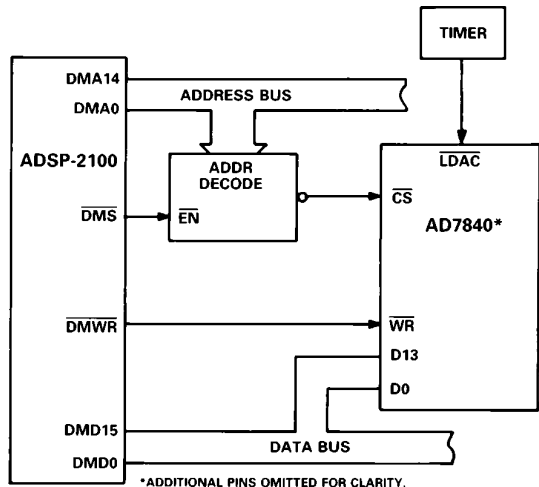
Figure 15. AD7840-ADSP-2100 Parallel Interface
