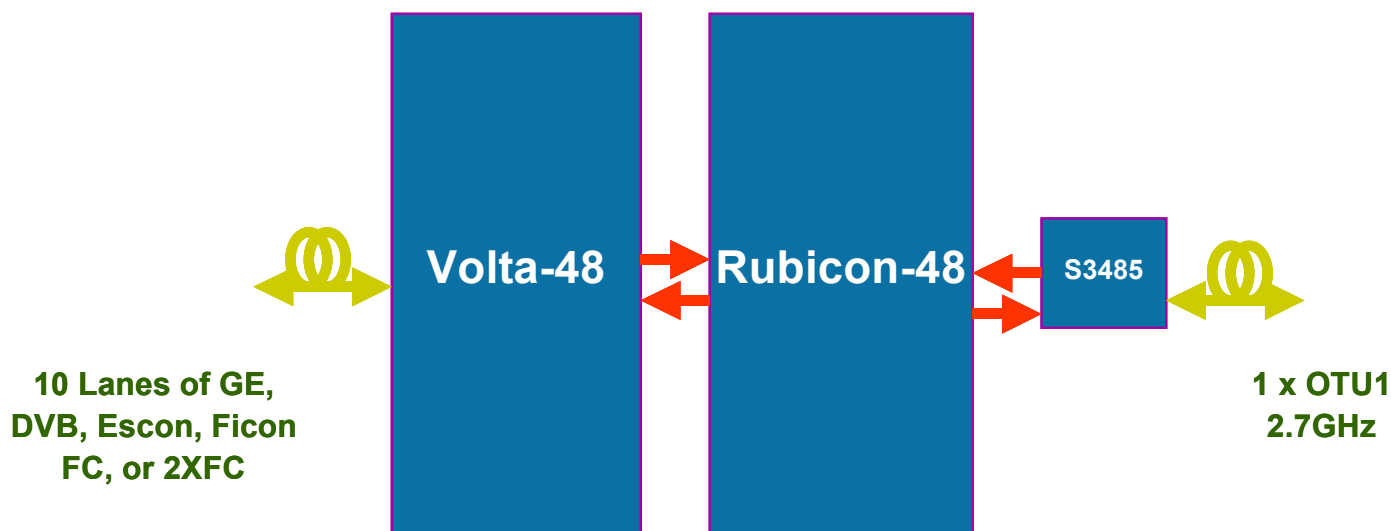
Figure 2: Multi-Protocol LAN Transport
