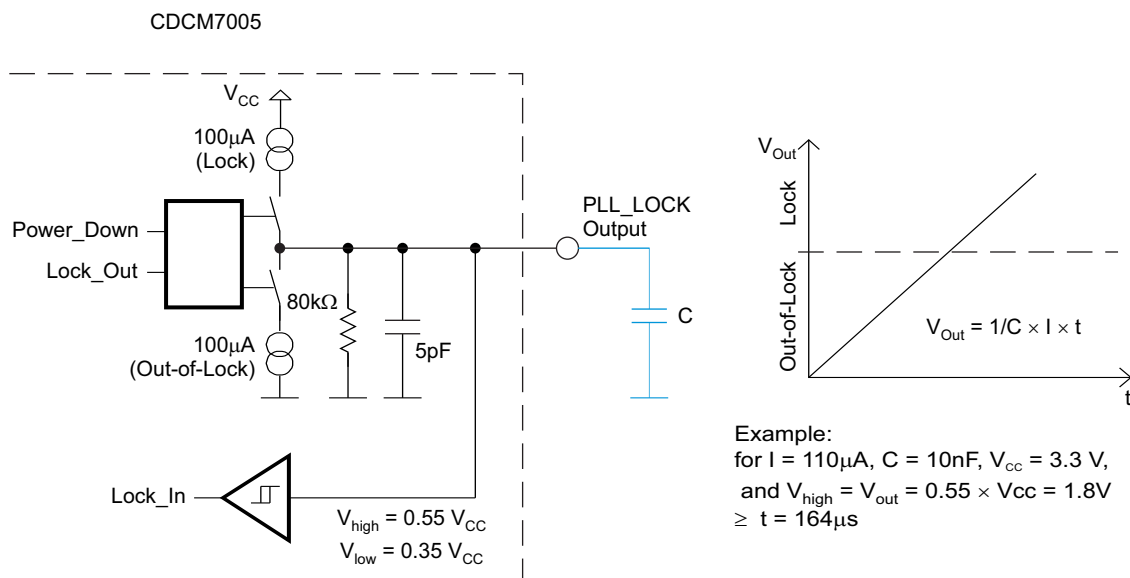
Figure 18. Analog Lock-Detect
