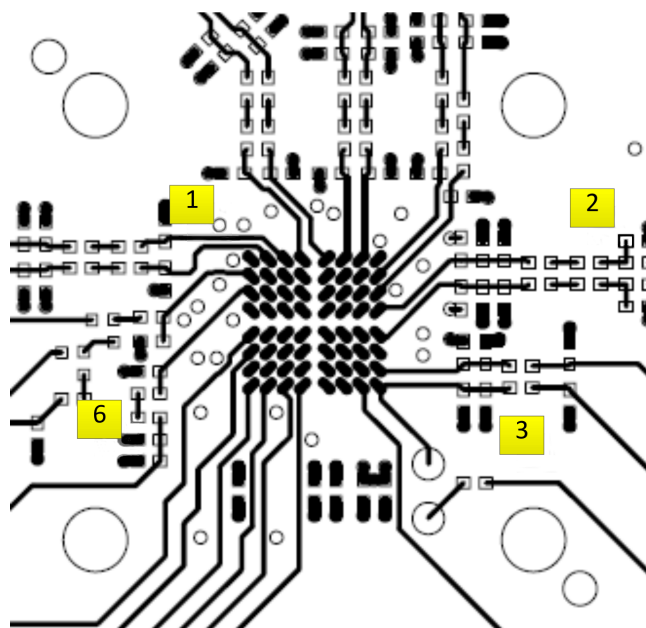
Top Plane
