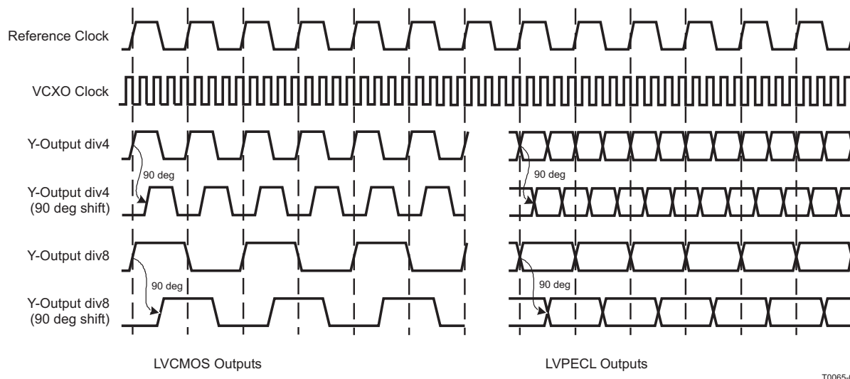
Figure 20. Output Switching Diagram
