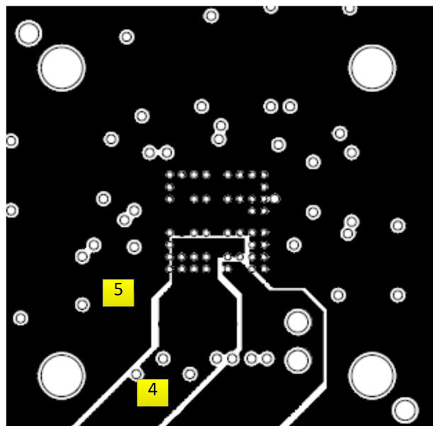
Power Plane
