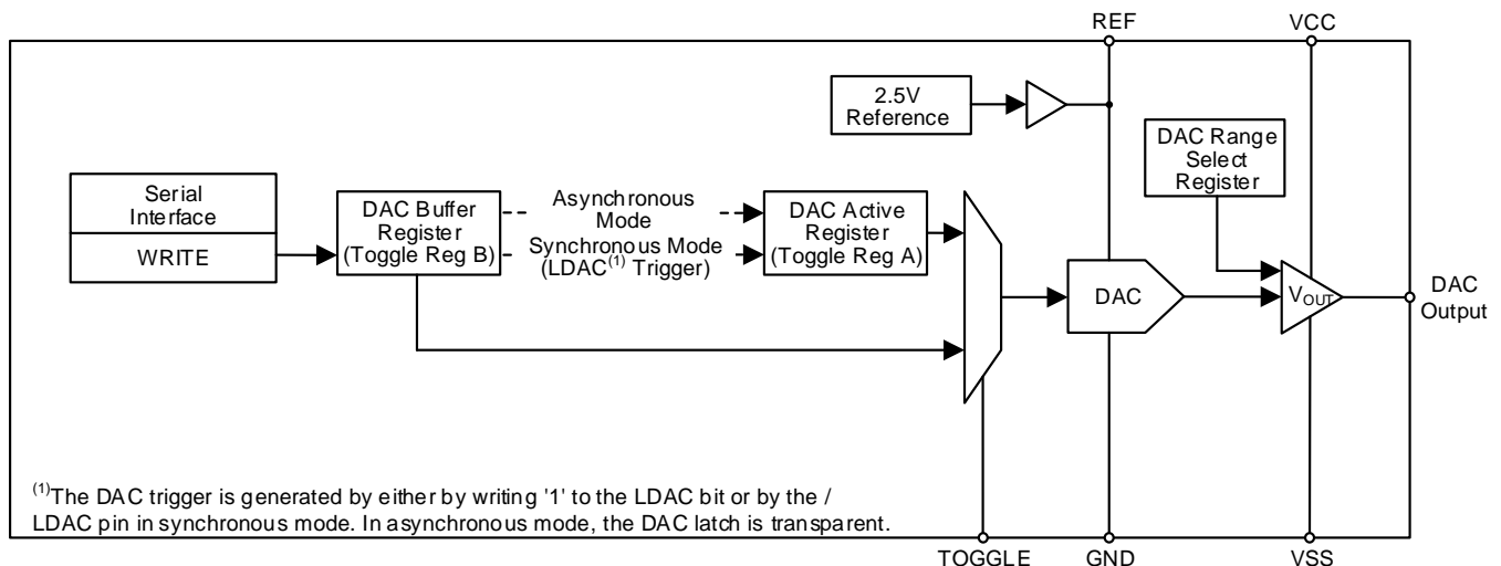
Figure 47. DACx1416 DAC Block Diagram
