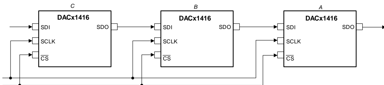
Figure 51. Daisy-Chain Layout
