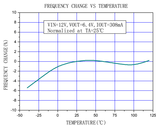
Figure10. Frequency change Curve
