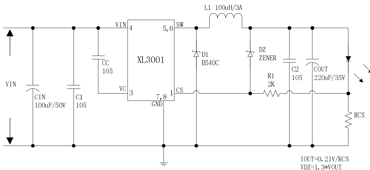
Figure19. XL3001 System Parameters Test Circuit (LED OVP)
