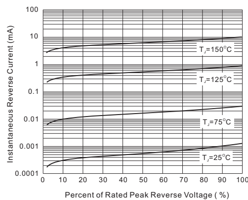
Fig. 4 - Reverse Characteristics
