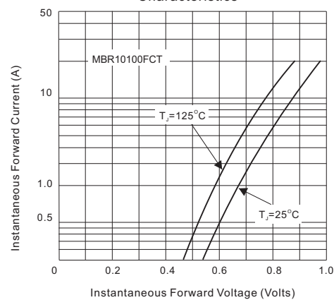
Fig. 3.2 - Instantaneous Forward Characteristics
