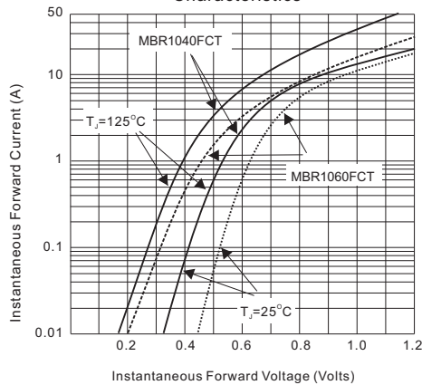
Fig. 3.3 - Instantaneous Forward Characteristics
