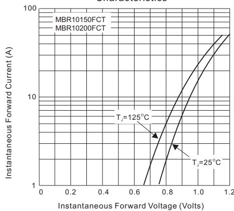
Fig. 3.3 - Instantaneous Forward Characteristics
