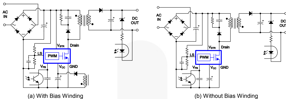
Figure 1. Typical Application
