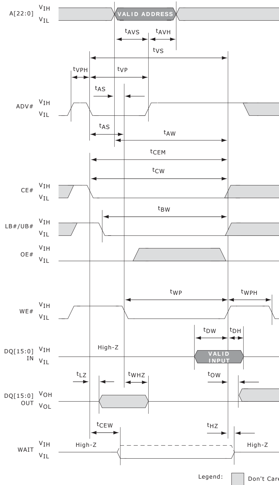
Figure 34.I4 Asynchronous Write Using ADV#
