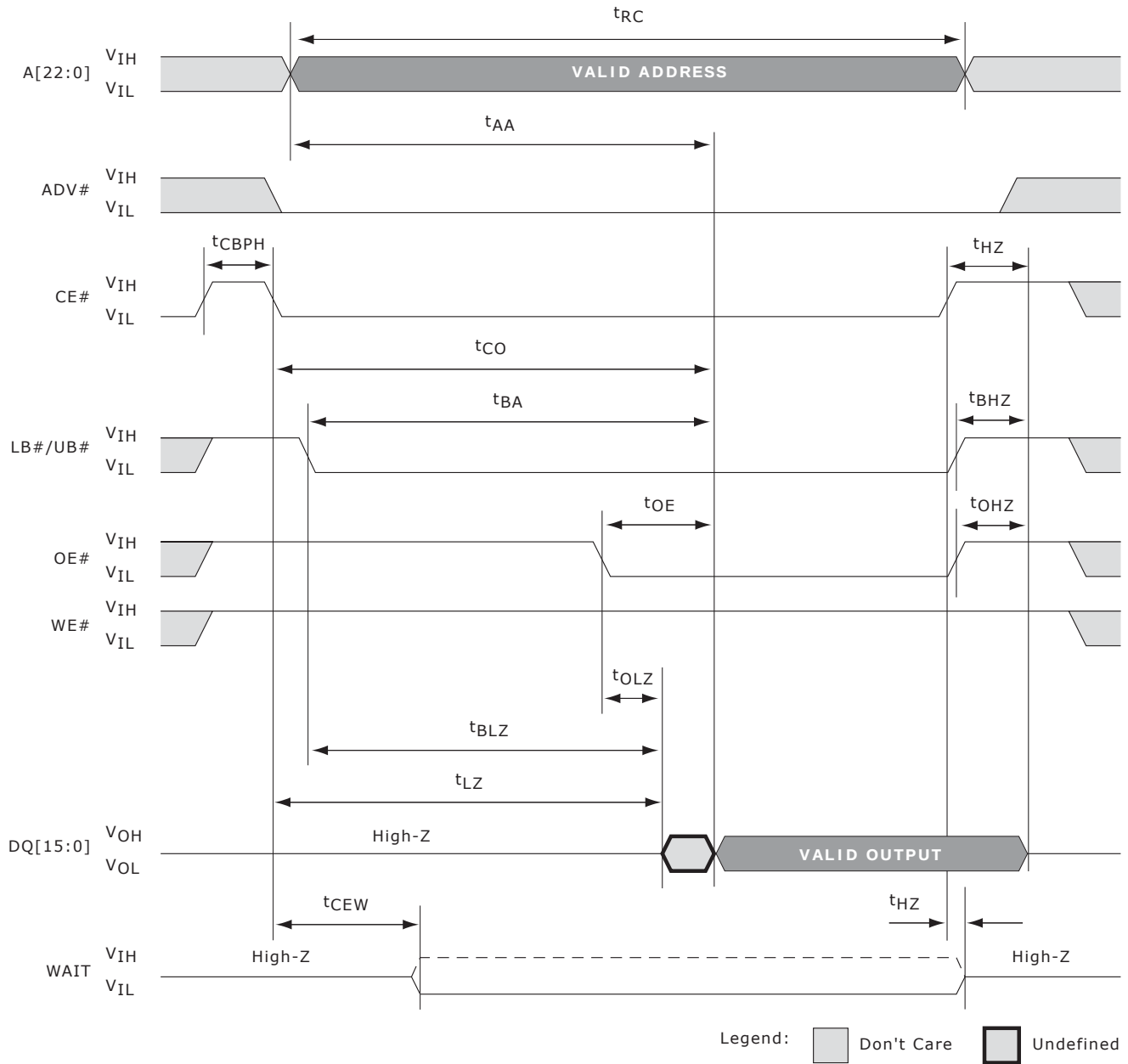
Figure 34.4 Asynchronous Read
