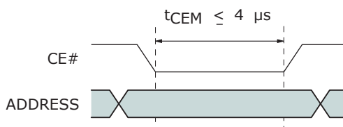
Figure 35.1 Extended Timing for t_{CEM}
