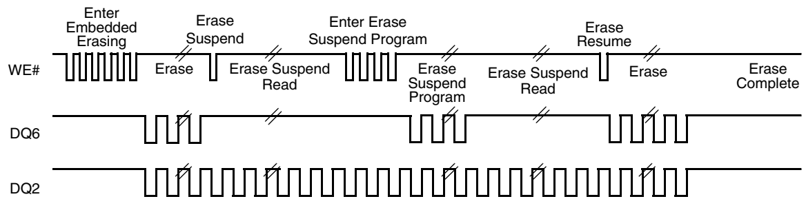
Figure 25.I5 Synchronous Data Polling Timings/Toggle Bit Timings
