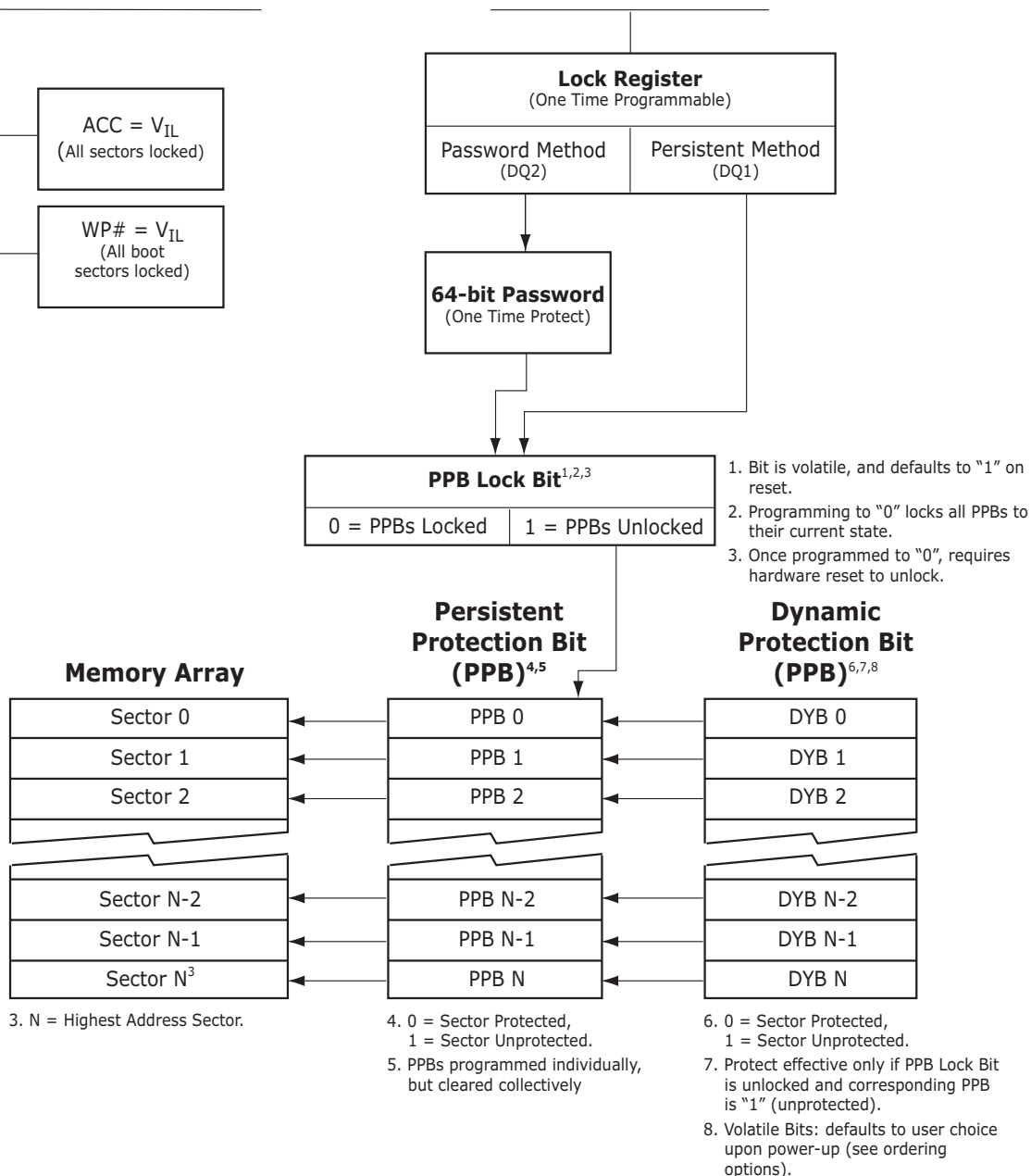
Figure 9.1 Advanced Sector Protection/Unprotection
