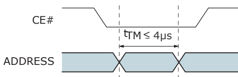
Figure 35.2 Extended Timing for t_{TM}
