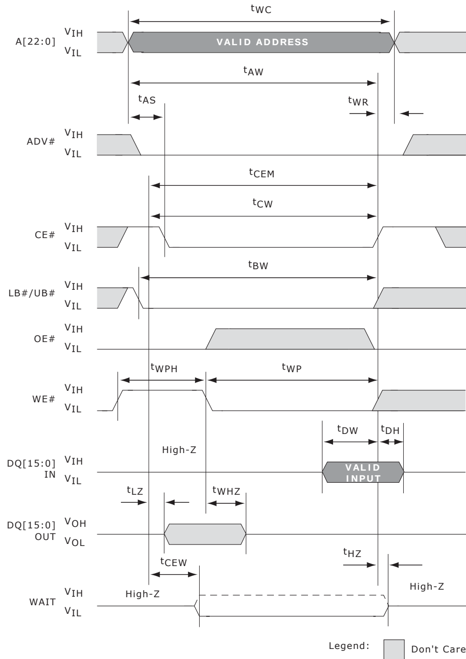
Figure 34.I2 LB#/UB#-Controlled Asynchronous Write
