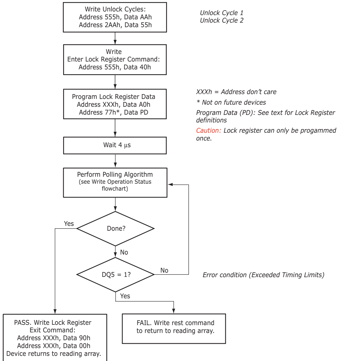
Figure 9.3 Lock Register Program Algorithm
