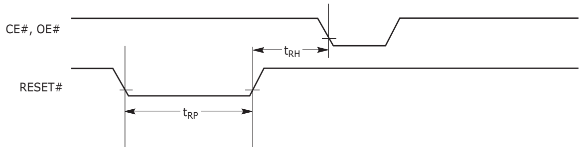
Figure I2.I2 Reset Timings
