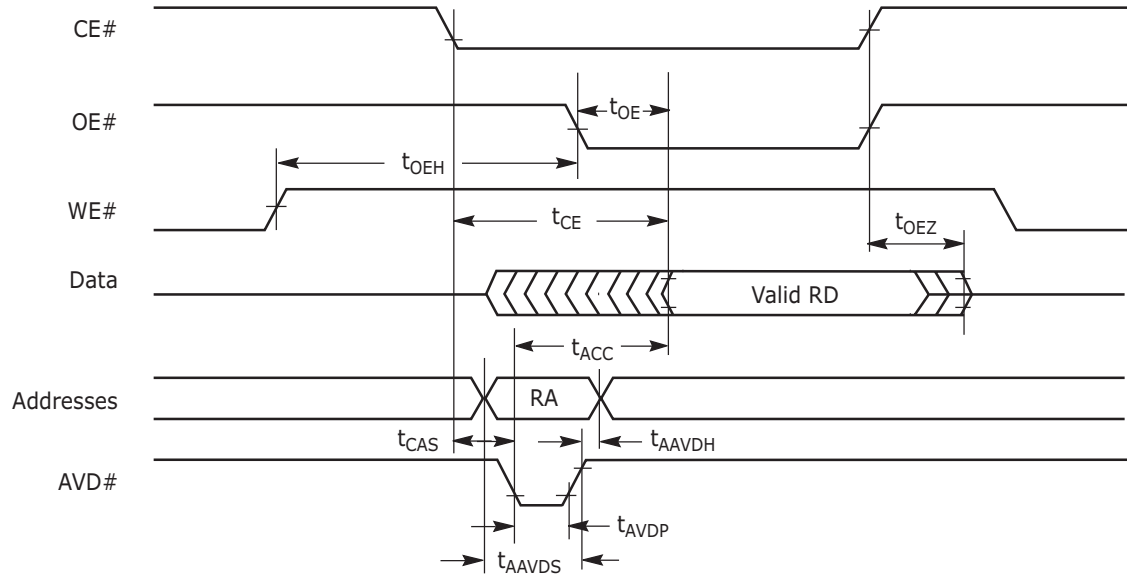
Figure I2.II Asynchronous Mode Read
