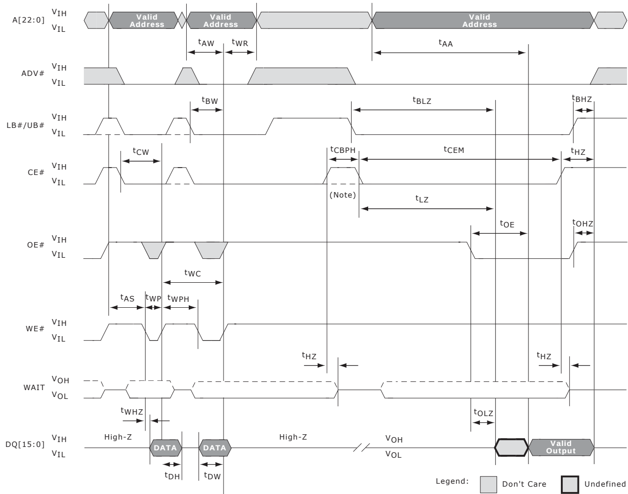
Figure 34.29. Asynchronous Write Followed by Asynchronous Read—ADV# Low
