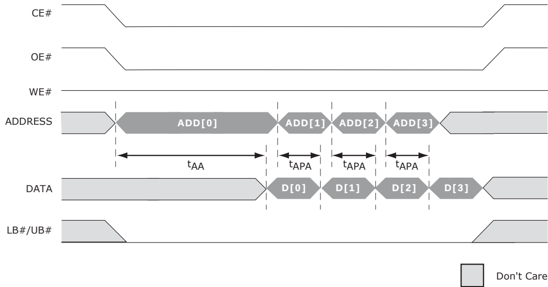
Figure 29.3 Page Mode Read Operation ( \text{ADV}\# Low)
