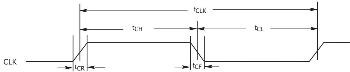
Figure 12.6 CLK Characterization
