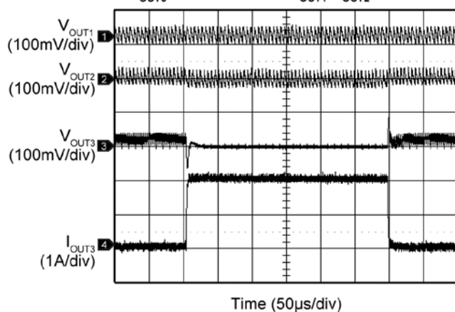
Transient Cross Regulation ( I_{OUT3} = 50\text{mA} to 2\text{A} , I_{OUT1}, I_{OUT2} = 20\text{mA} )
