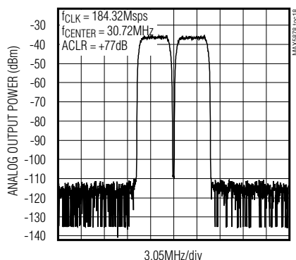
ACLR FOR W-CDMA MODULATION TWO CARRIER ACLR
