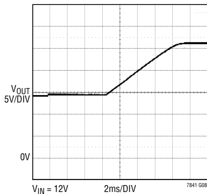
Soft Start-Up
