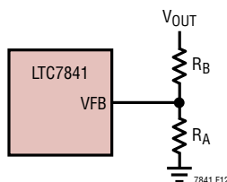
Figure 12. Setting Output Voltage
