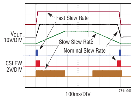
Output Voltage Changes with MFR\_VOUT\_COMMAND
