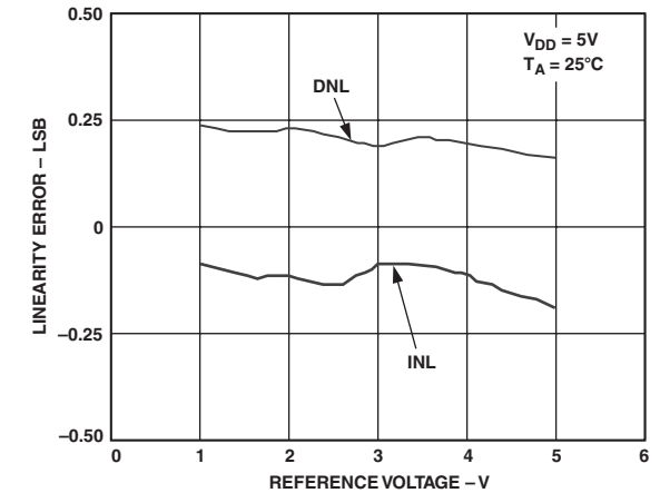
TPC 21. Linearity Error vs. Reference Voltage
