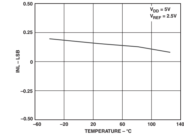
TPC 17. Integral Nonlinearity vs. Temperature
