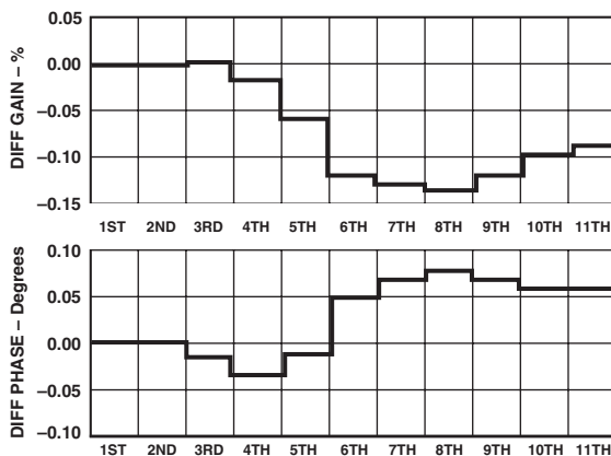
TPC 44. Differential Gain and Phase @ V_S = \pm 5\text{ V} ; R_L = 1\text{ k}\Omega
