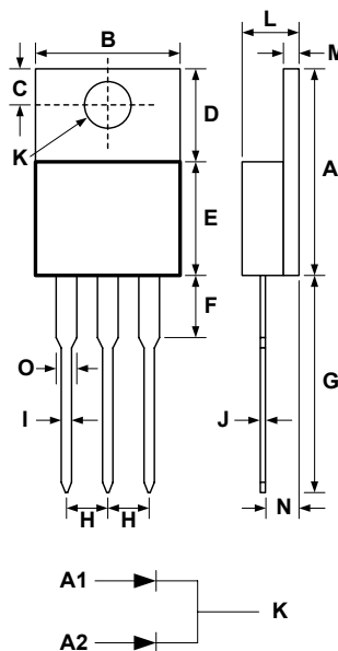
TO-220AB
