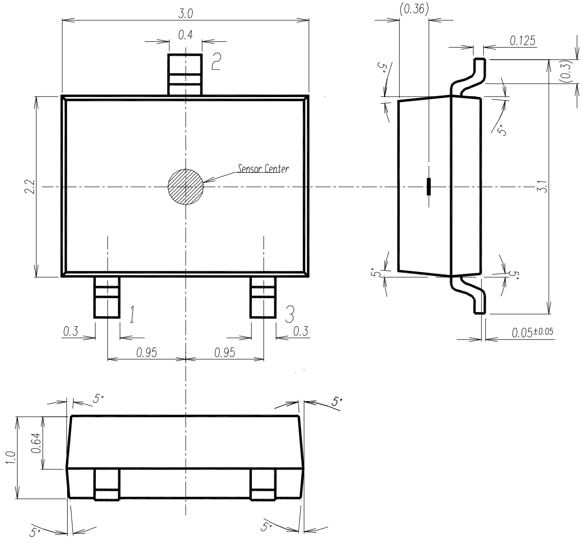
Figure 11. Outline Dimensions
