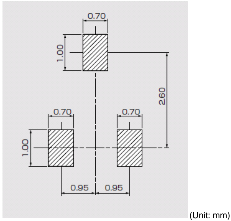
Figure 12. Land Pattern
