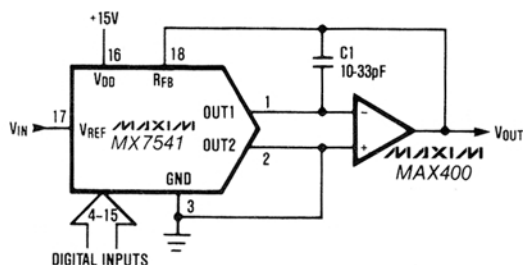
Unipolar Operation
