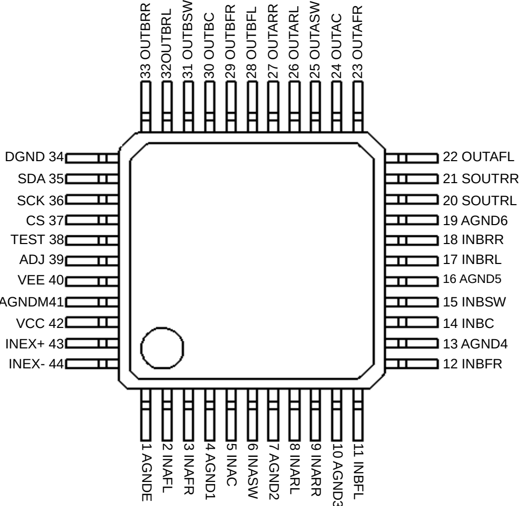
TOP VIEW
