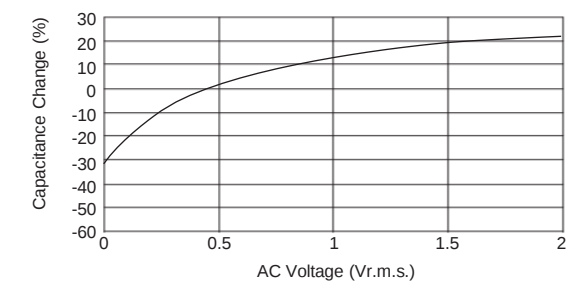
[Example of AC Voltage Characteristics] Sample: X7R(R7) Characteristics 10 \mu F, Rated Voltage 6.3VDC
