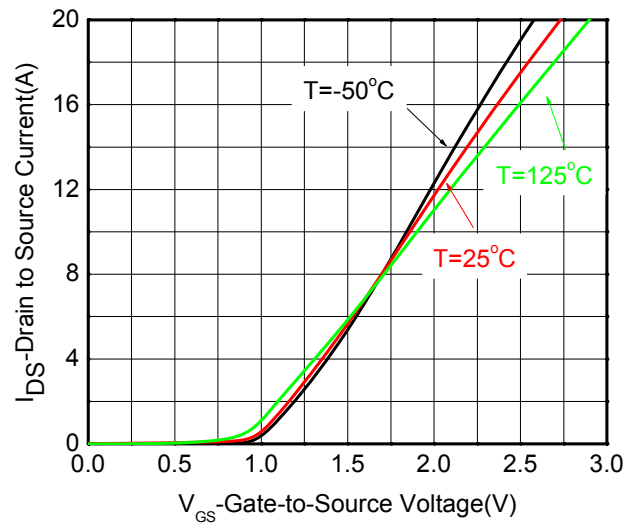
Transfer characteristics
