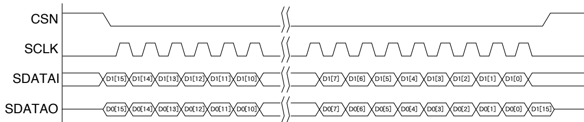
Assignment of volume control data
