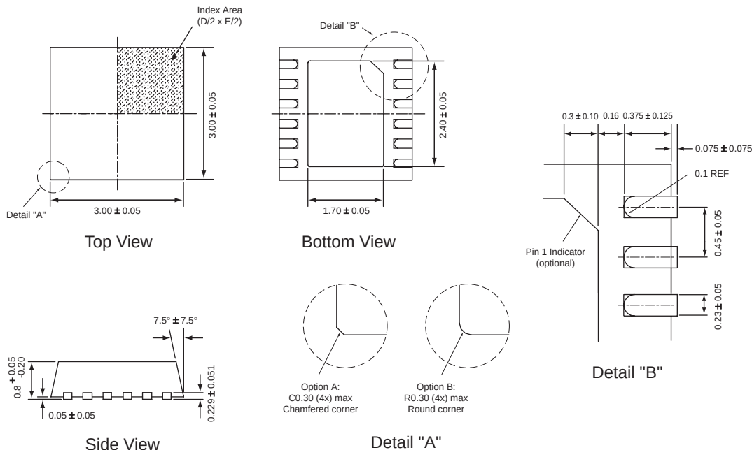
TDFN33-12
