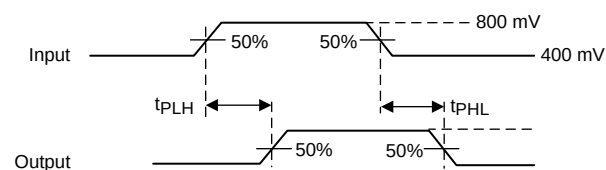
Figure 10. Propagation Delay
