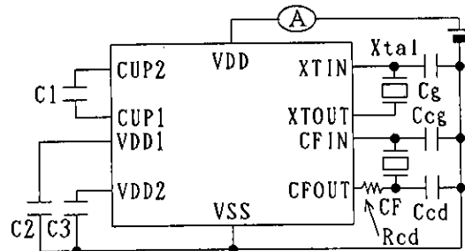
Figure 8 Supply Current Test Circuit
