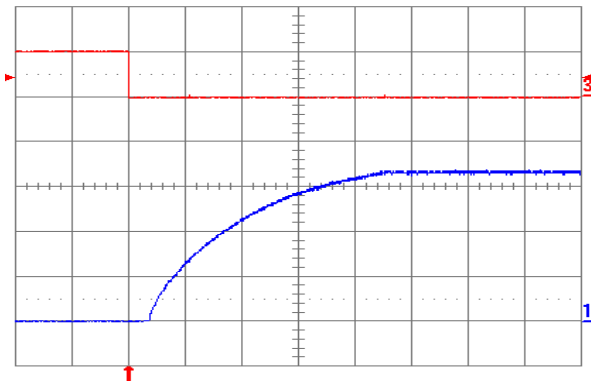
Figure 3.3V.16. Turn-on transient at full rated load current (resistive) plus 10,000 \mu\text{F} at V_{in} = 48\text{ V} , triggered via ON/OFF pin. Top trace: ON/OFF signal (5 V/div.). Bottom trace: output voltage (1 V/div.). Time scale: 2 ms/div.
