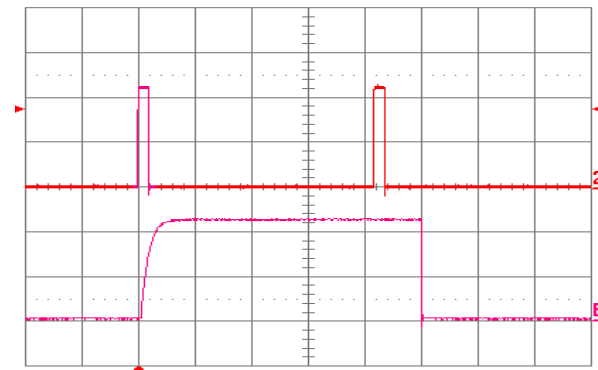
Figure 1.5V.24. Load current (top trace, 20 \text{ A}/\text{div} , 50 \text{ ms}/\text{div} ) into a 10 \text{ m}\Omega short circuit during restart, at V_{in} = 48 \text{ V} . Bottom trace ( 20 \text{ A}/\text{div} , 2 \text{ ms}/\text{div} ) is an expansion of the on-time portion of the top trace.
