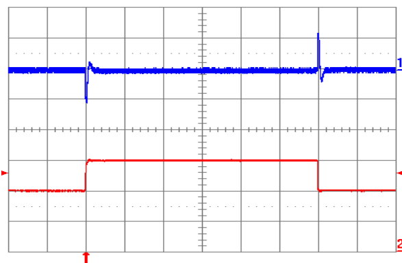
Figure 1.5V.18. Output voltage response to load current step-change (20 A - 30 A - 20 A) at V_{in} = 48\text{ V} . Top trace: output voltage (100 mV/div.). Bottom trace: load current (10 A/div.). Current slew rate: 5 A/ \mu\text{s} . C_o = 470\text{ }\mu\text{F POS} + 1\text{ }\mu\text{F} ceramic. Time scale: 0.2 ms/div.
