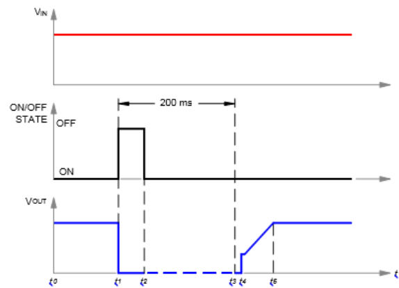
Figure 7. Startup scenario #3.
