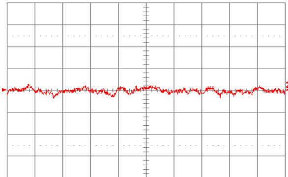
Figure 1.2V.22. Input reflected ripple current, i_s (10 mA/div.), measured through 10 \mu\text{H} at the source at full rated load current and V_{in} = 48 \text{ V} . Refer to Fig. 1.2V.20 for test setup. Time scale: 1 \mu\text{s}/\text{div.}
