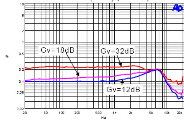
12. THD+N vs Frequency ( P_o=3\text{W} )
