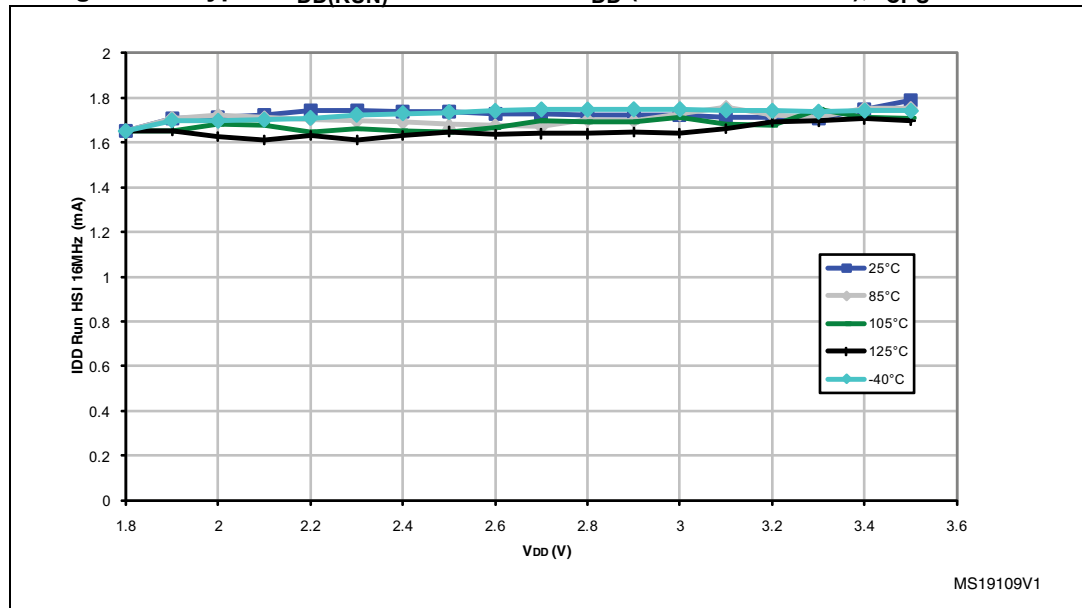
Figure 13. Typical I_{DD(RUN)} from RAM vs. V_{DD} (HSI clock source), f_{CPU} = 16 MHz
