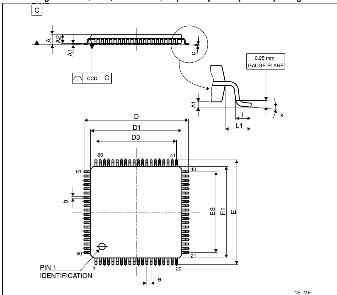
Figure 47. LQFP80, 14 x 14 mm, 80-pin low profile quad flat package
