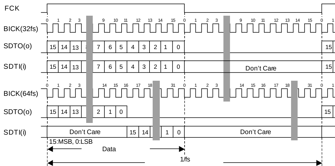
Figure 25. Mode 1 Timing
