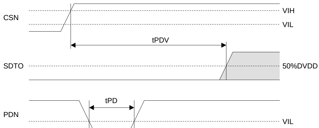
Figure 14. Power Down &amp; Reset Timing
