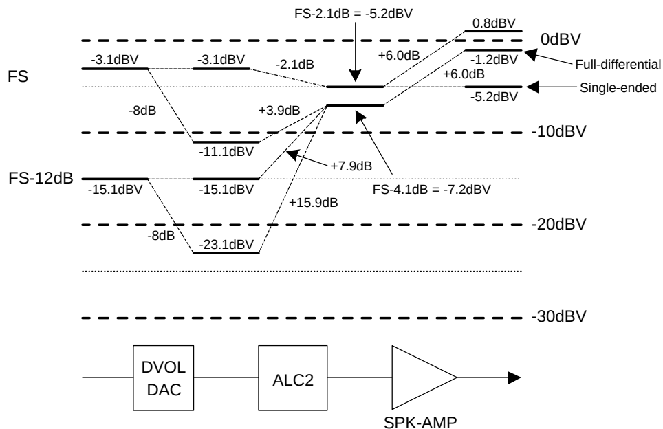
Figure 30. Speaker-Amp Output Level Diagram (SVDD=3.3V, DVOL= -8.0\text{dB} , SPKG bit = “0”)
