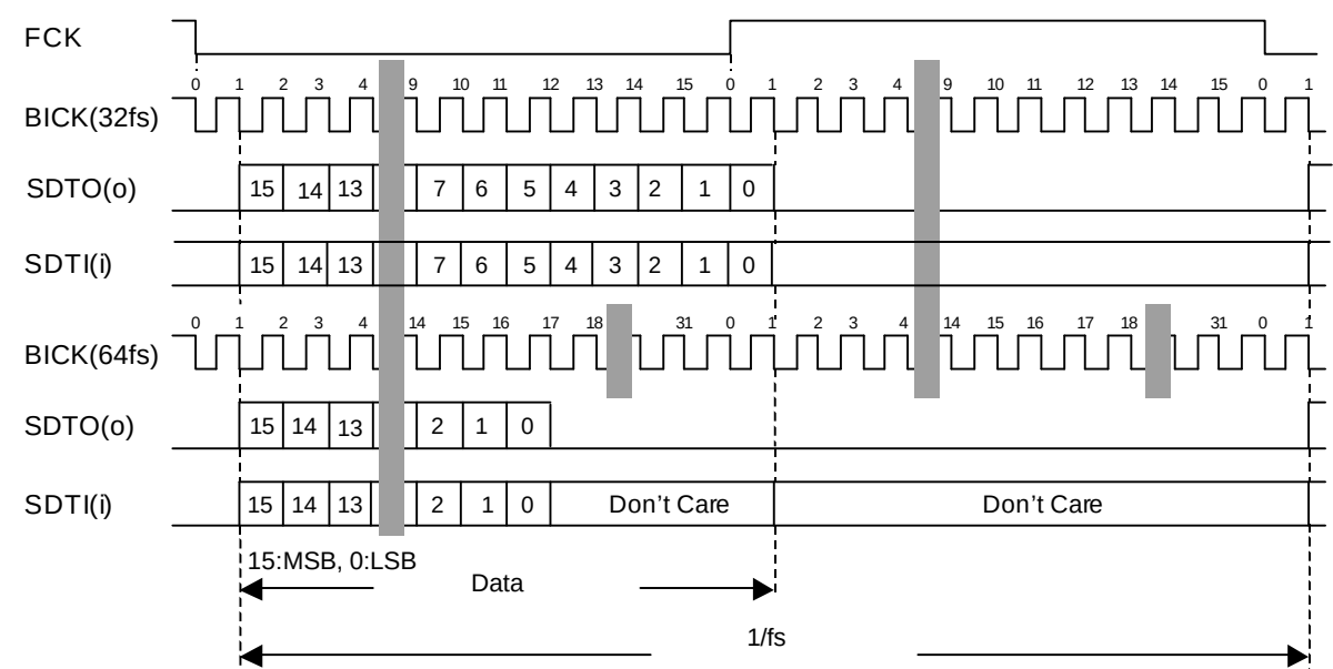
Figure 27. Mode 3 Timing
