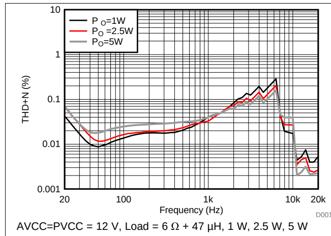
Figure 1. THD+N vs Frequency (BTL)
