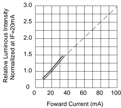
FIG.4 RELATIVE RADIANT INTENSITY VS. FORWARD CURRENT
