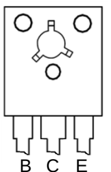
Front Face View Pin-Out
