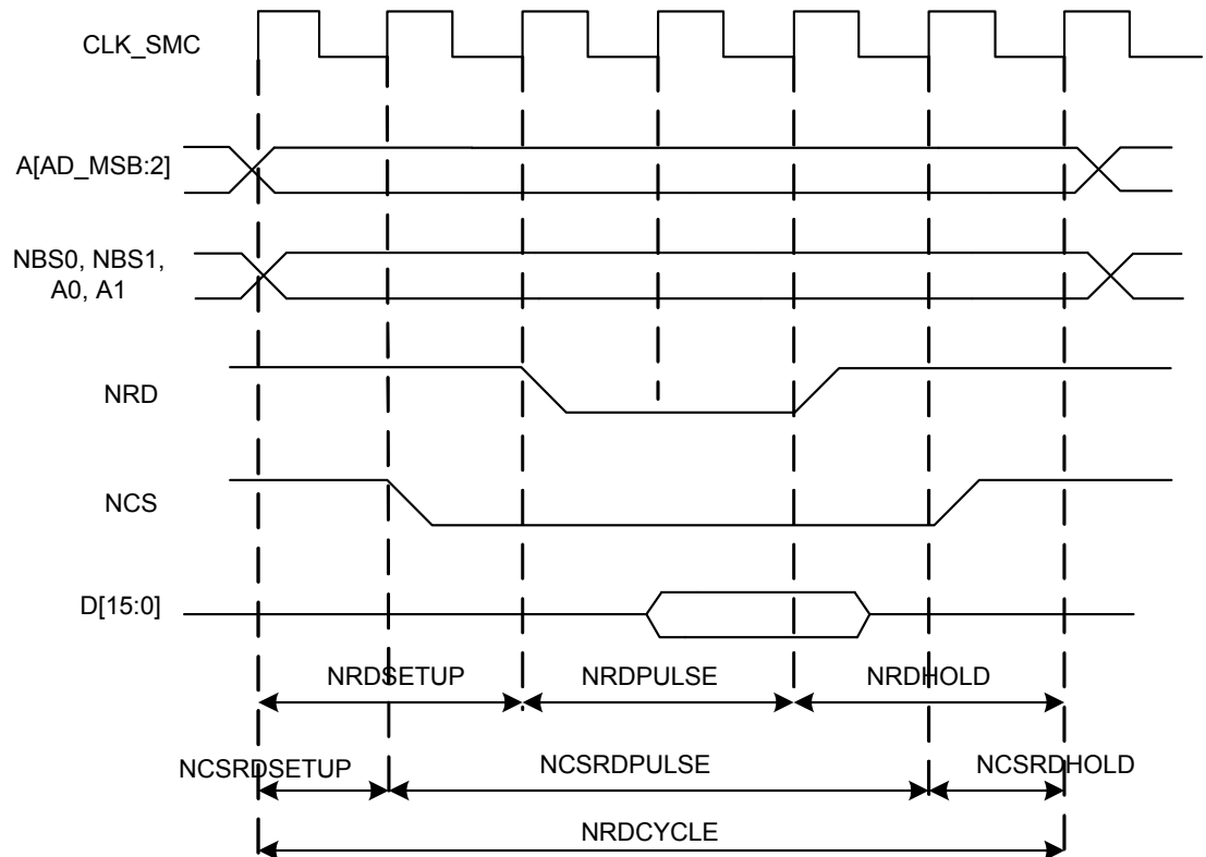
Figure 15-7. Standard Read Cycle
