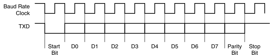
Figure 25-5. Character Transmit
