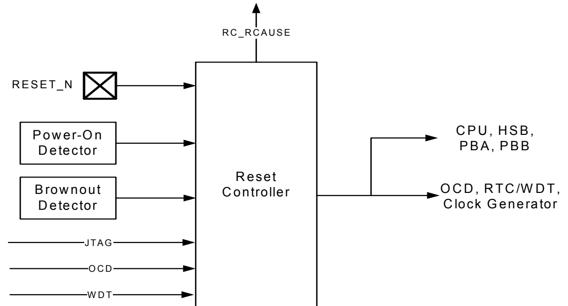
Figure 7-6. Reset Controller Block Diagram
