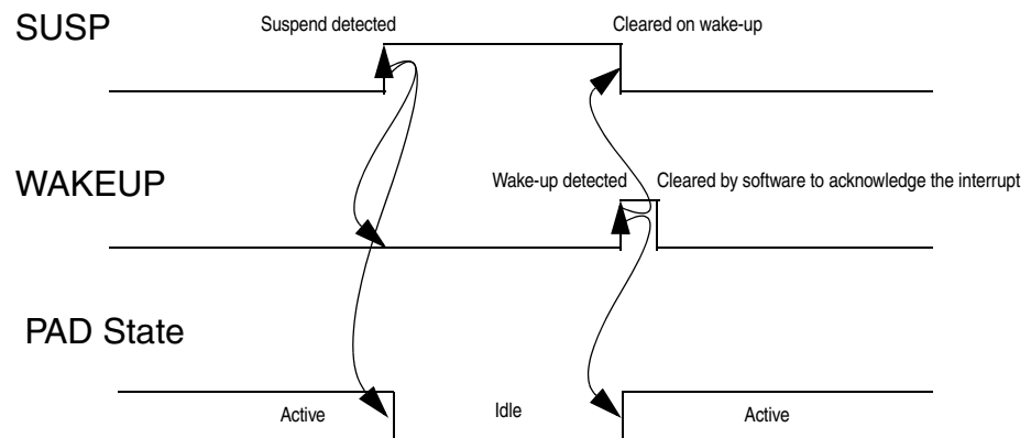
Figure 26-9. Pad Events
