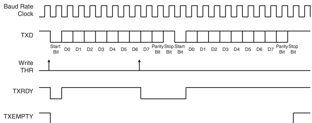
Figure 25-6. Transmitter Status
