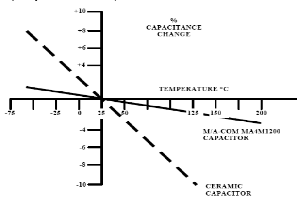
TYPICAL CAPACITANCE CHANGE FOR MNS and CERAMIC CAPACITOR vs TEMPERATURE (200 pF CAPACITOR)
