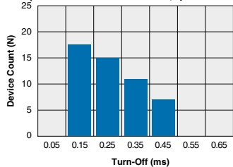
IAA110P Typical Turn-Off Time (N=50 Ambient Temperature = 25°C) (Load Current = 100mADC; I_F = 5\text{mA} )
