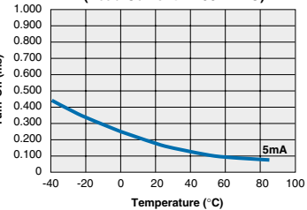
IAA110P Typical Turn-Off vs. Temperature (Load Current = 100mADC)
