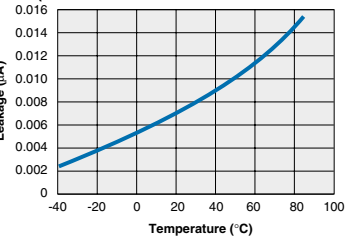
IAA110P Typical Leakage vs. Temperature (Measured across Pins 14 & 16 or 11 & 13)
