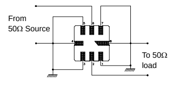
Test Circuit
