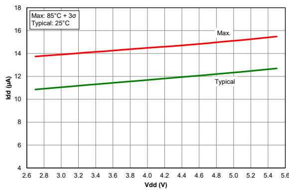
Figure 39-68. I_{PD} , Low-power Brown-out Reset, LPBOR = 0, PIC18F27/47K40 only
