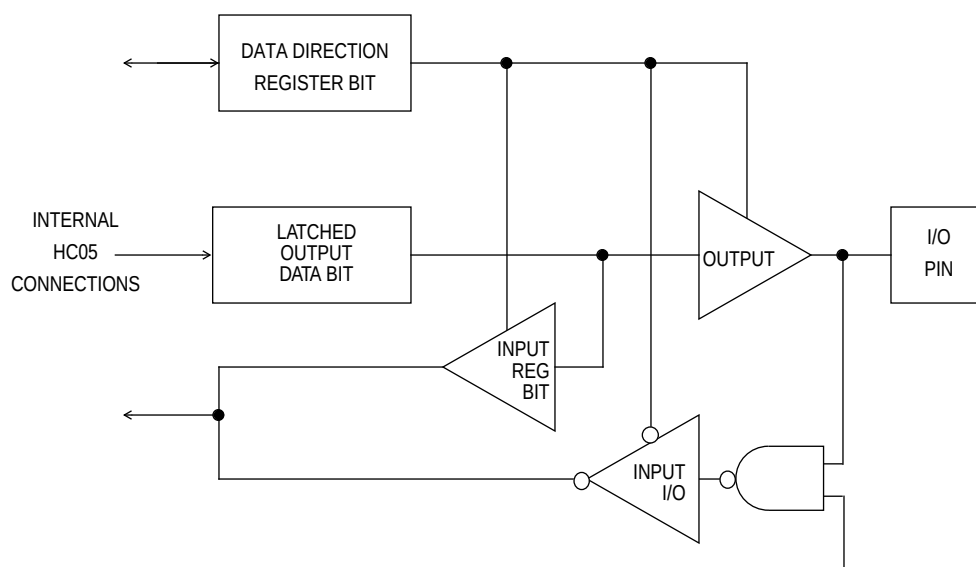
Figure 7-2. I/O Circuitry
