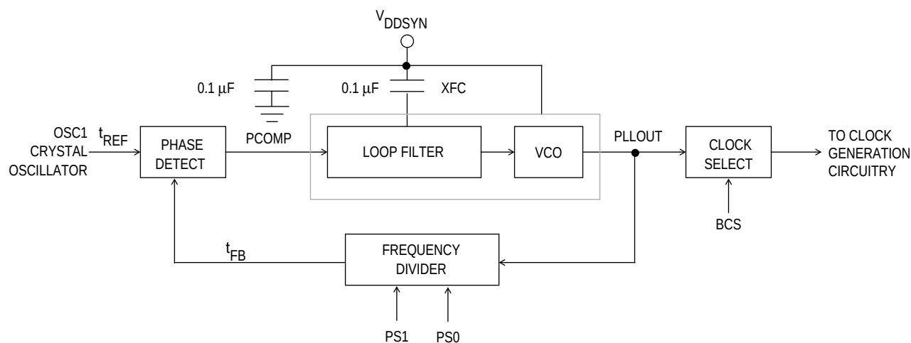
Figure 10-1. PLL Circuit
