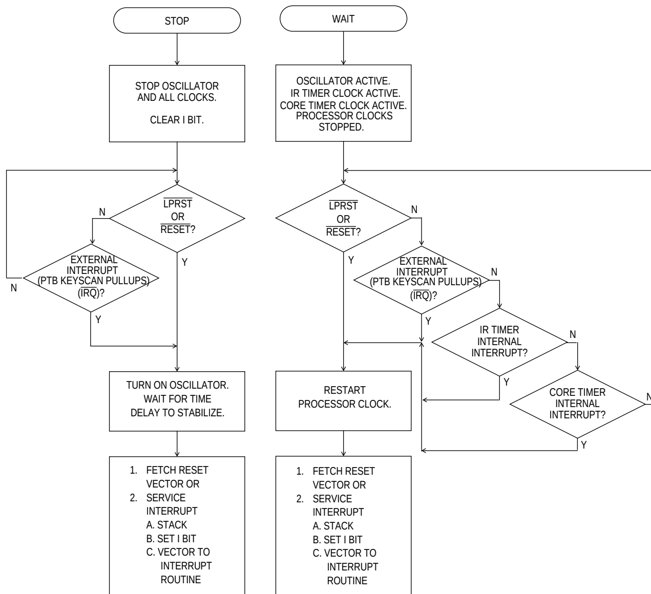
Figure 6-2. Stop/Wait Flowchart
