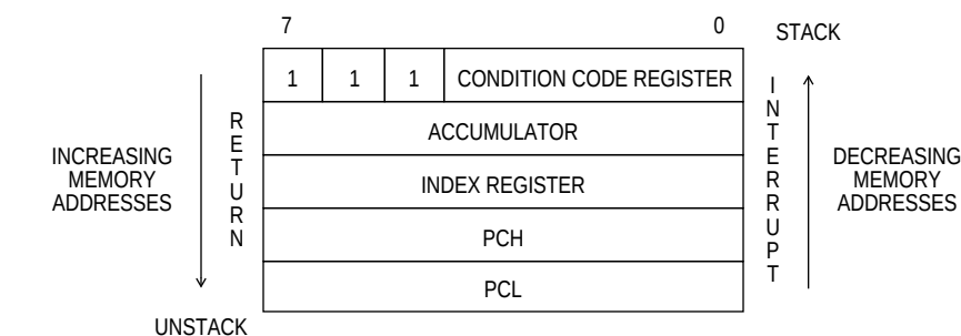
Figure 3-1. Programming Model
