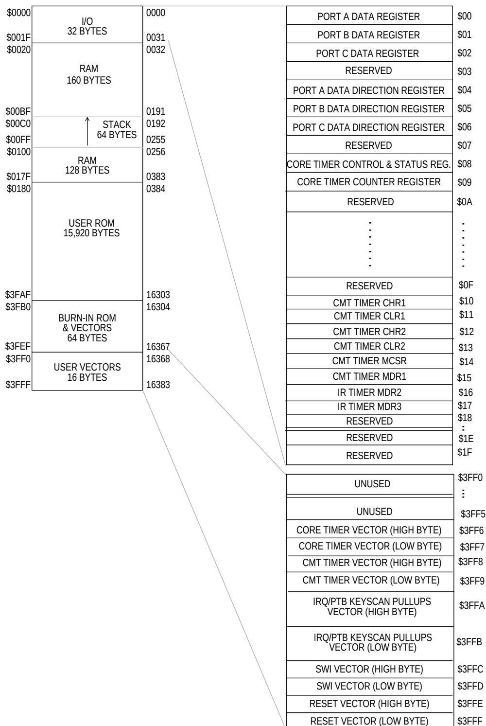
Figure 2-1. MC68HC05RC17 Memory Map
