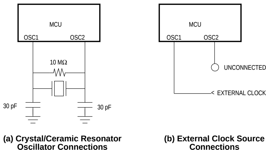
Figure 1-4. Oscillator Connections
