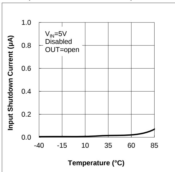
Input Shutdown Current vs. Temperature
