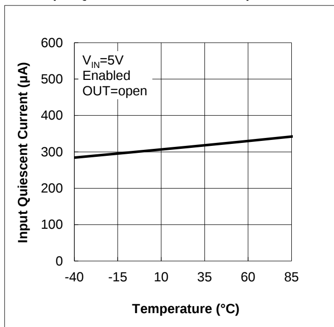
Input Quiescent Current vs. Temperature
