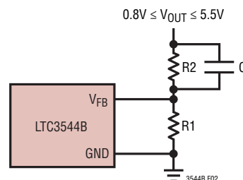
Figure 2. Setting the LTC3544B Output Voltage
