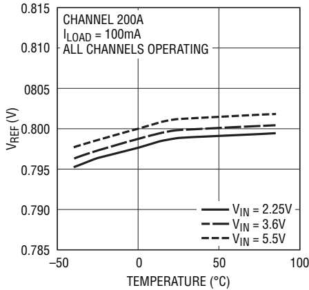
V_{REF} vs Temperature at 2.25V, 3.6V, 5.5V
