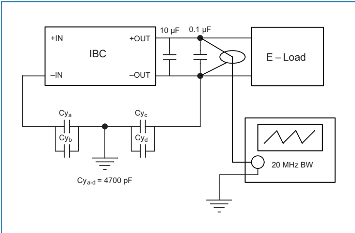
Figure 23 — Test circuit; output voltage ripple
