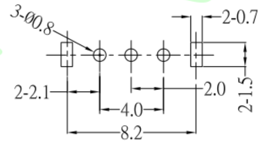
P.C.B MOUNTING PATTERN
