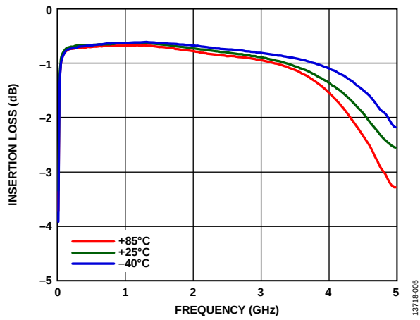
Figure 5. Insertion Loss vs. Frequency over Temperature, V_{DD} = 3\text{ V} , V_{CTL} = 3\text{ V}
