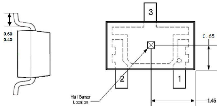
Hall Plate Chip Location (Bottom view)
