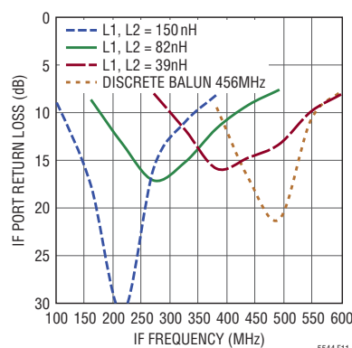
Figure 11. IF Output Return Loss
