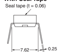
Flat Actuator With Seal Tape
