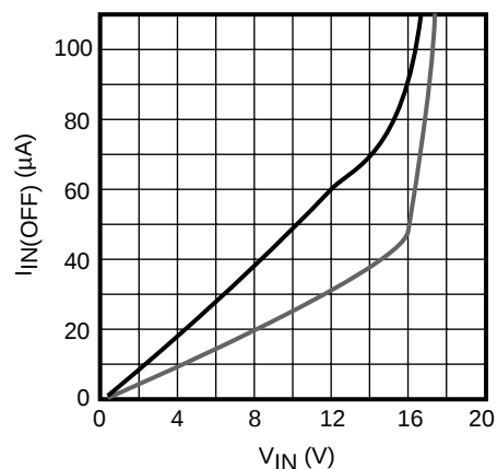
INPUT CURRENT (SHUTDOWN) vs. INPUT VOLTAGE
