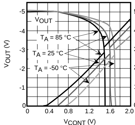
OUTPUT VOLTAGE AND CONTROL CURRENT vs. CONTROL VOLTAGE
