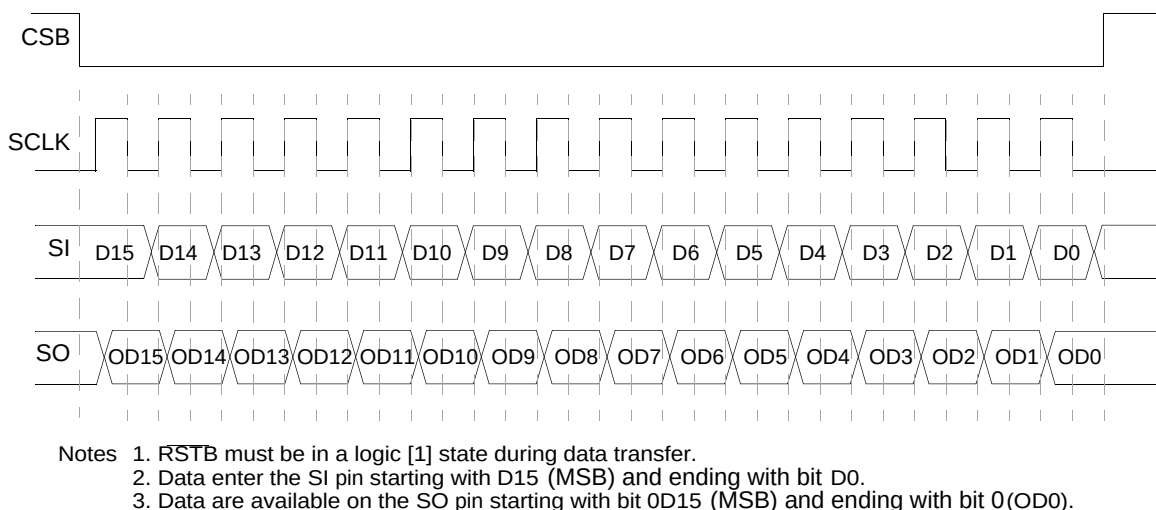
Figure 20. 16-Bit SPI Interface Timing Diagram
