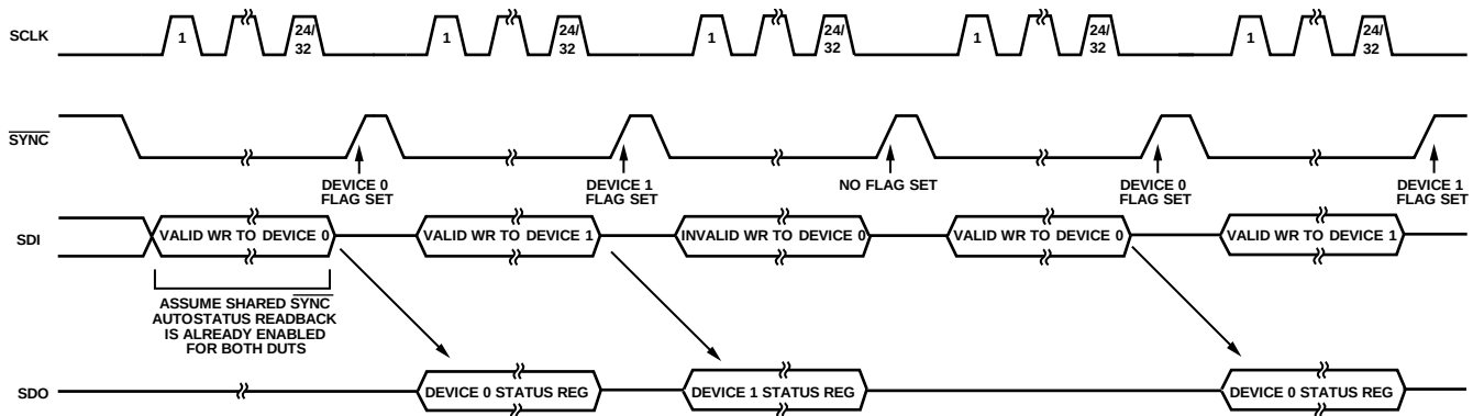
Figure 91. Shared/ SYNC Autostatus Readback Example
