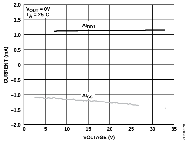
Figure 70. ALDD1/ALSS Current vs. AVDD1/AVSS Supply
