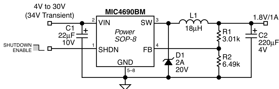
1.8V Adjustable Converter
