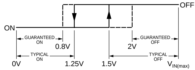
Shutdown Hysteresis
