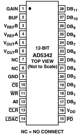
AD5342 PIN CONFIGURATION
