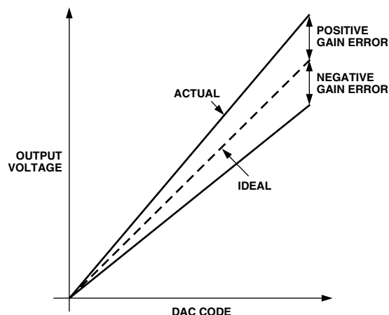
Figure 2. Gain Error
